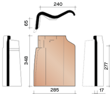
P4517080 3.6 pieces/Lm Left facade tile
