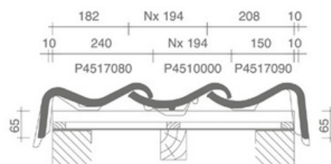
Cross-section roof with double well pan
