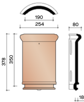
P0003100 3 pieces/Lm Semicircular North Pole - 190 mm
