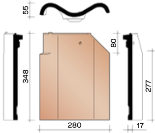
P4518050 3.6 pieces/Lm Double Well Pan
