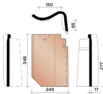
P4517090 3.6 pieces/Lm Right facade tile
