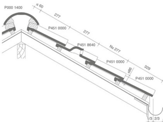
Length-section roof at the height of frost without closure 1400 with ventilation pan-mortarred
