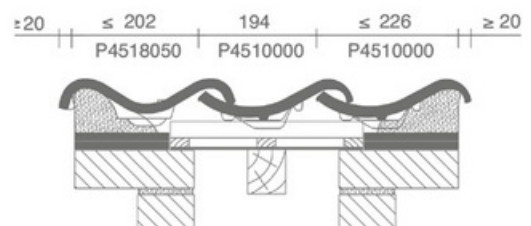
Cross-section roof with double well pan
