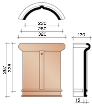
P0001200 3 pieces/Lm Semicircular frost/northern tree - 225 mm
