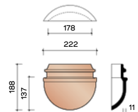
P0003110 Semicircular North Pole - 190 mm
